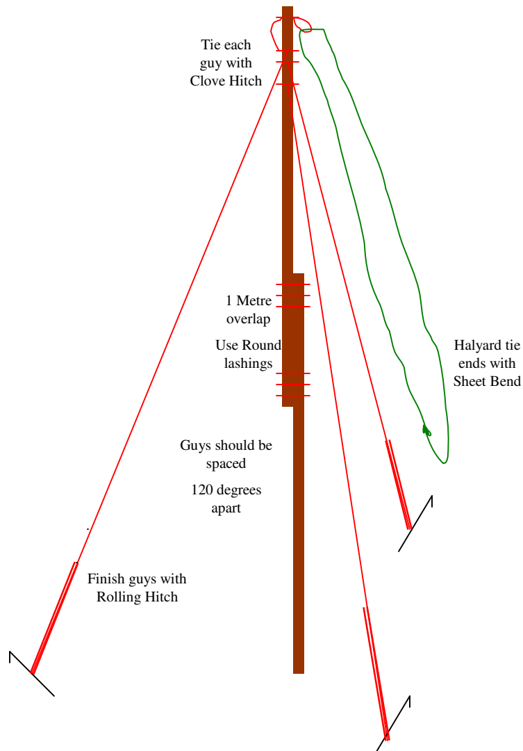
Basic 5 Meter Flagpole (Mast) using two 3 Metre poles.
